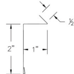
⑭ ABS Counter Flashing (ABSCFcc)
