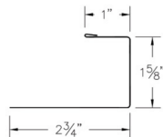
⑧ ABS Starter "J" (ABSSJcc)
