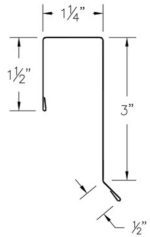
② ABS Rake Trim (ABSRtcc)
