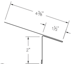
⑥ ABS Residential Eave (ABSRcc)
