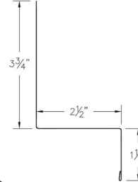
⑤ ABS Sidewall (ABSSWcc)
