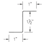
⑪ ABS Metal "Z" Closure (ABSZcc)
