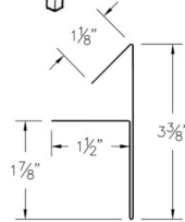
④ ABS Slim Line Rake (ABSSLRcc)
